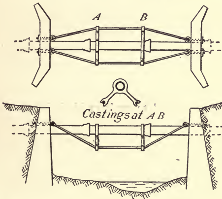
FIG. 30.—SEWER CROSSING CREEK ABOVE WATER.
